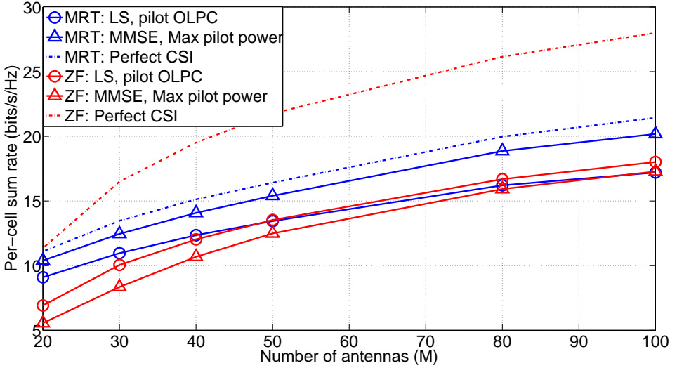
Figure 5.8: Effect of channel estimation technique on sun rate. MMSE performs better than LS with MRT , but under-performs LS with ZF. We use pilot OLPC with LS to keep channel estimation error below 0 dB. ( L = 21, U = 1 )
