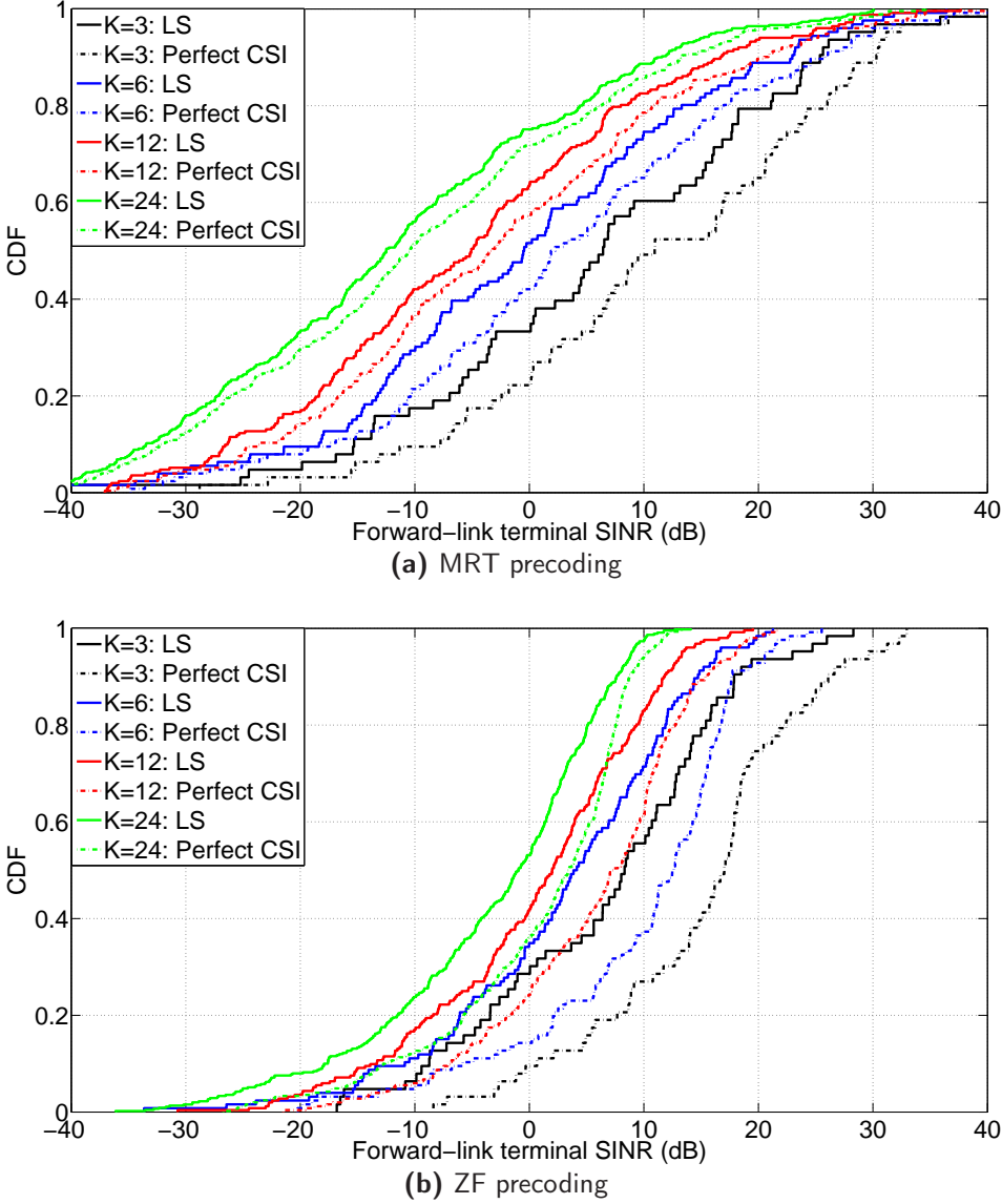
Figure 5.5: Impact of pilot contamination on forward-link terminal SINR with pilot OLPC, LS estimation and linear precoding ( L = 21, U = 1, M = 100 )
