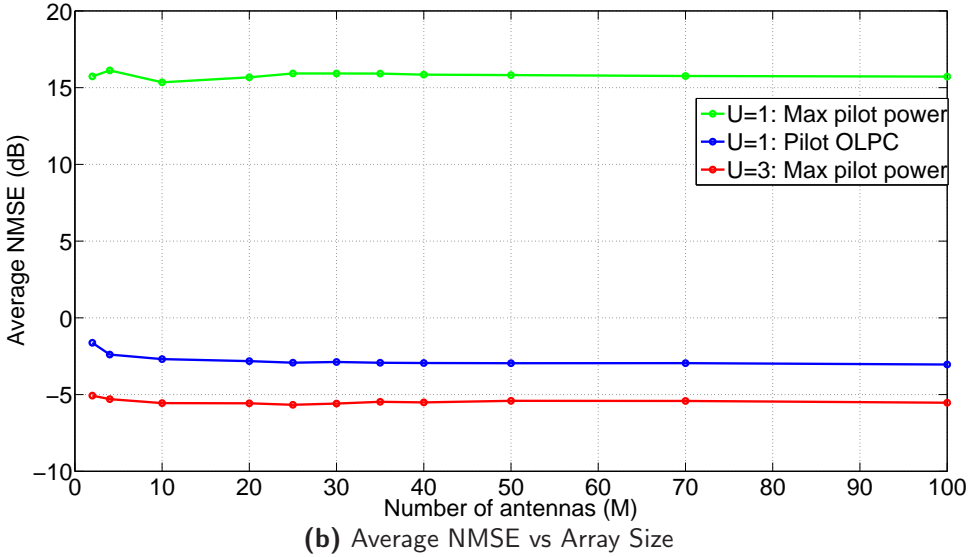
Figure 5.9: Effect of less aggressive pilot reuse on NMSE of LS channel estimation. The pilot contamination is effectively mitigated, even in the absence of pilot OLPC ( L = 21, K = 12 )
