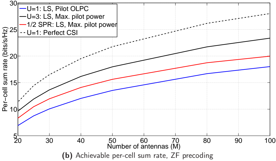
Figure 5.13: Forward-link SINR and rate for soft pilot reuse (SPR) with LS channel estimation ( L = 21, K = 12, M = 100 )
