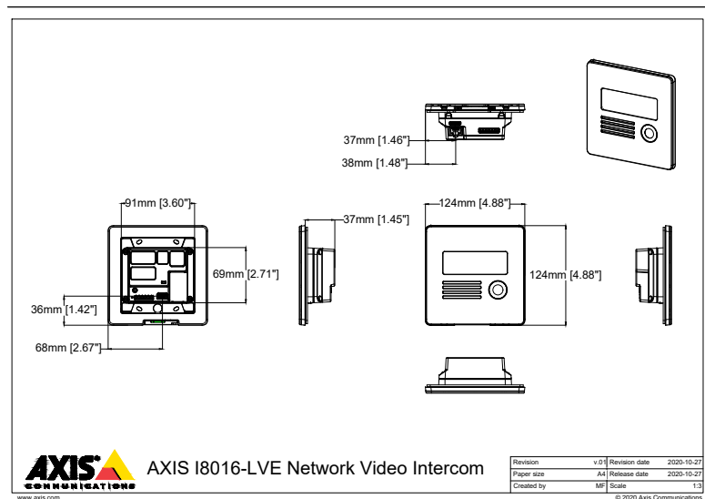
(b) Dimensions of Device 1
