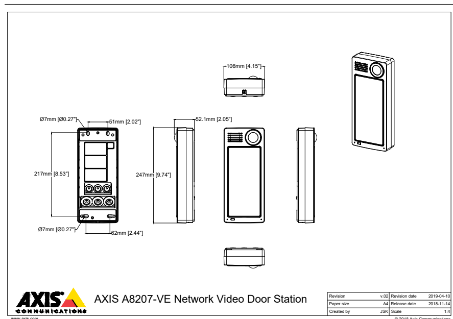
(b) Dimensions of Device 2
