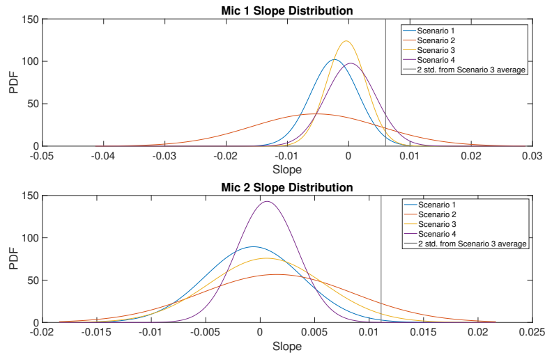
Figure 4.6: Average slope distribution for each scenario for 5 ms signal - Device 1
