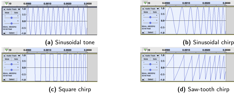
Figure 3.4: Different types and shapes of the signals used (the unit for the time axis is second)
