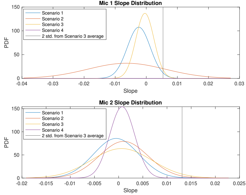
Figure 4.5: Average slope distribution for each scenario for 3 ms signal - Device 1
