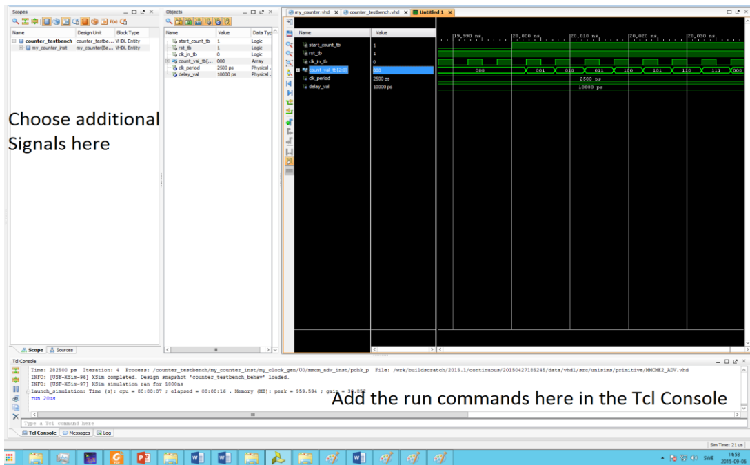
Figure 7: Simulation window
