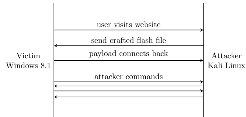
Figure 1: Overview of the attack performed in Metasploit.
