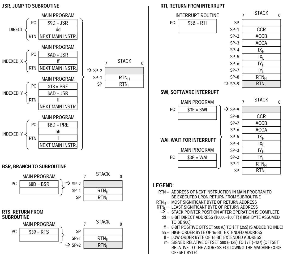
Figure 3-2. Stacking Operations
