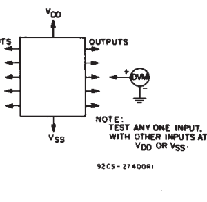
Fig. 21 - Noise immunity test circuit.
