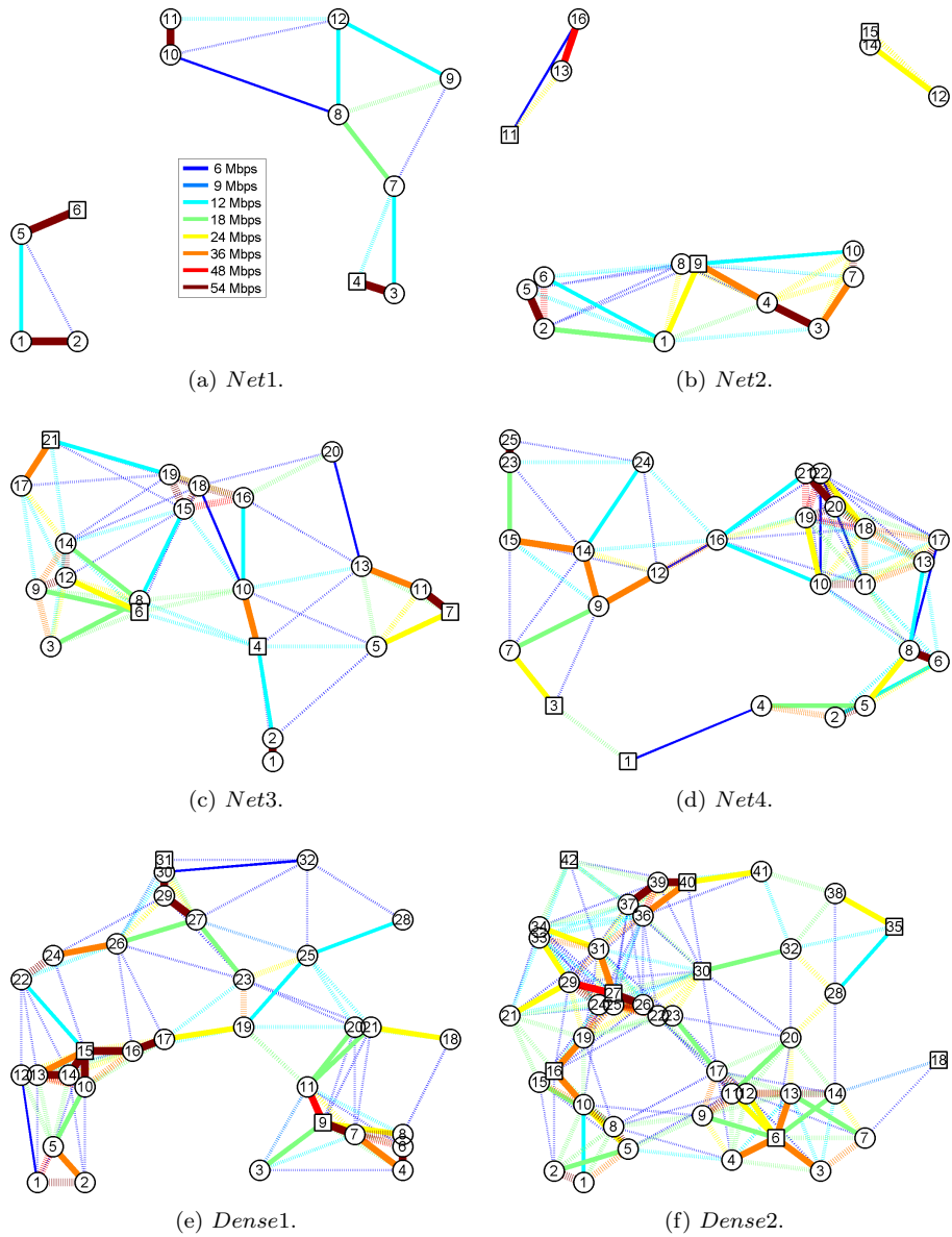
Figure 2: Tested networks.
