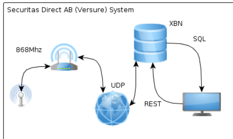
Figure 5.1: The System architecture of Securitas Direct AB (Versure)
