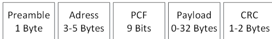
Figure 5. The Enhanced Shockburst packet divided into its five segments.
