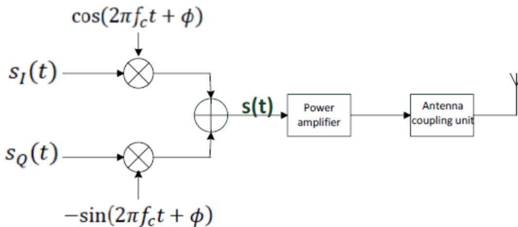
Figure 8. Block diagram illustrating frequency up-conversion (mixer stage) to the carrier frequency ( K is odd), the power amplifier, and the antenna coupling unit. The OFDM signal s(t) is given in equation (4.1).
