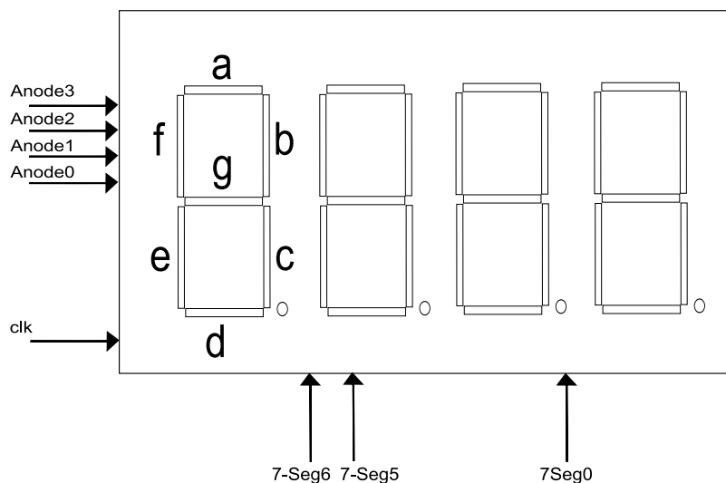
Figure 3: 7-segment display
